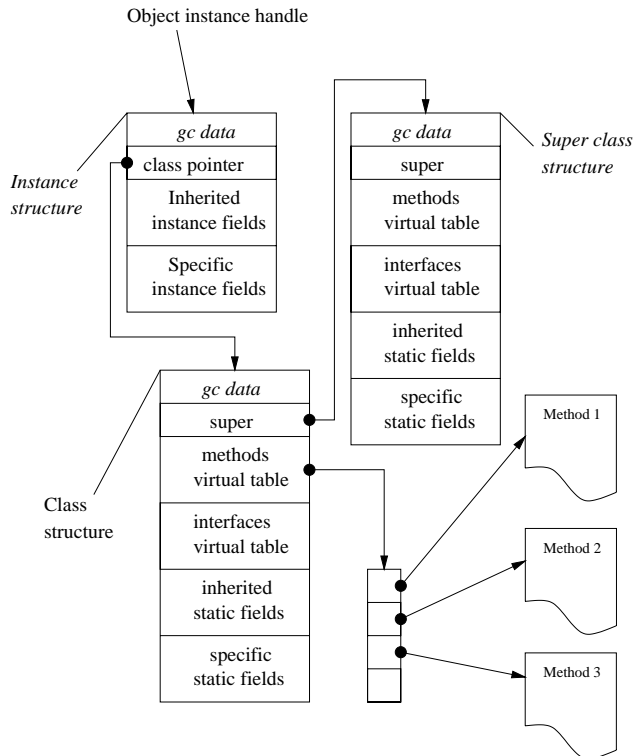
Figure 1. Run-time model of an object.
