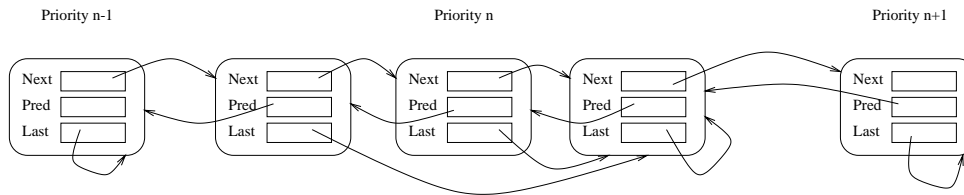
Figure 2. Queue data structure
